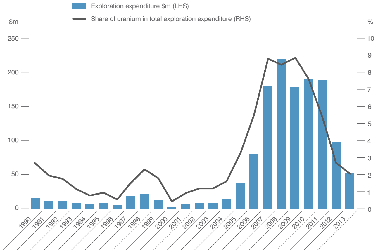
CHART 3 Uranium exploration expenditure in Australia
