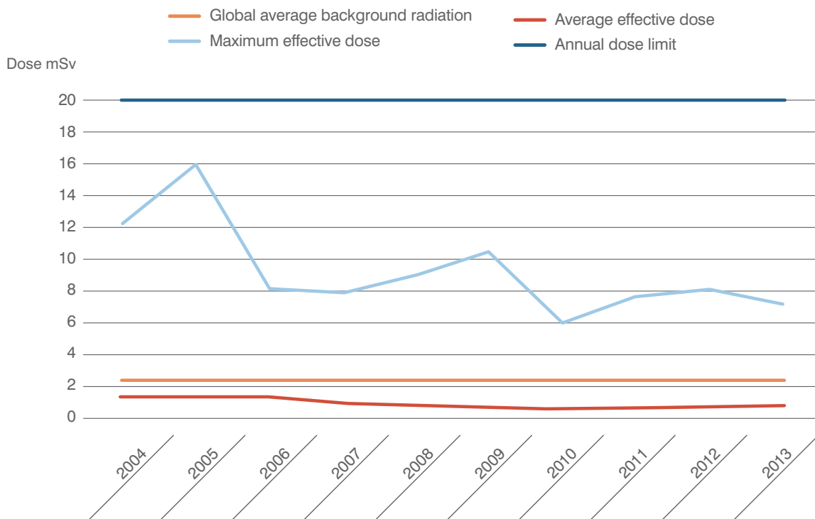
CHART 13 Average and maximum effective dose trends for Australian uranium mine workers, 2004-13
