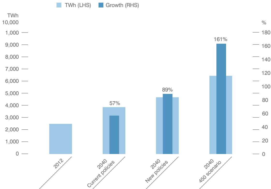
CHART 9 International Energy Agency nuclear energy projections 2012-2040
